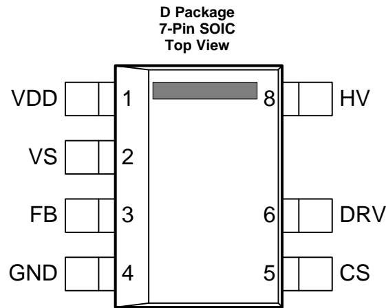
Pin Functions
