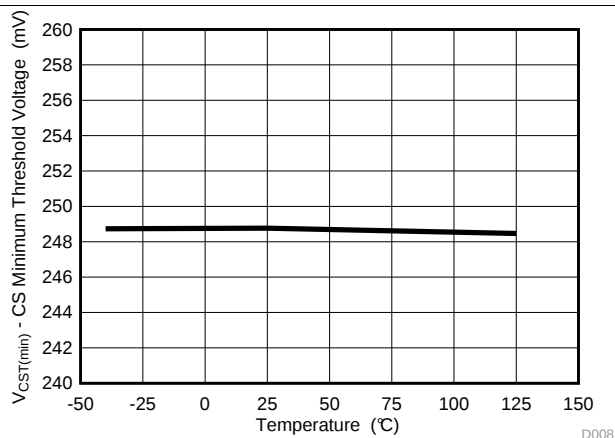
Figure 8. CS Minimum Threshold Voltage vs. Temperature
