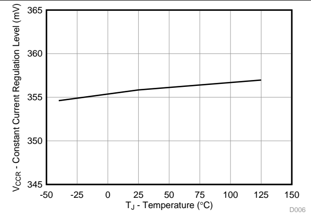
Figure 6. Constant-Current Regulation Level vs. Temperature
