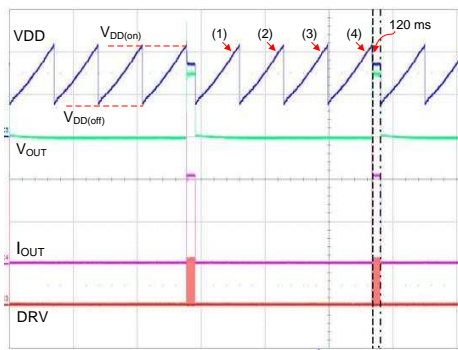
Figure 28. Soft-Short Protection
