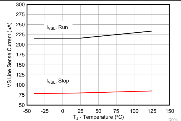
Figure 4. Line-Sense Current vs. Temperature
