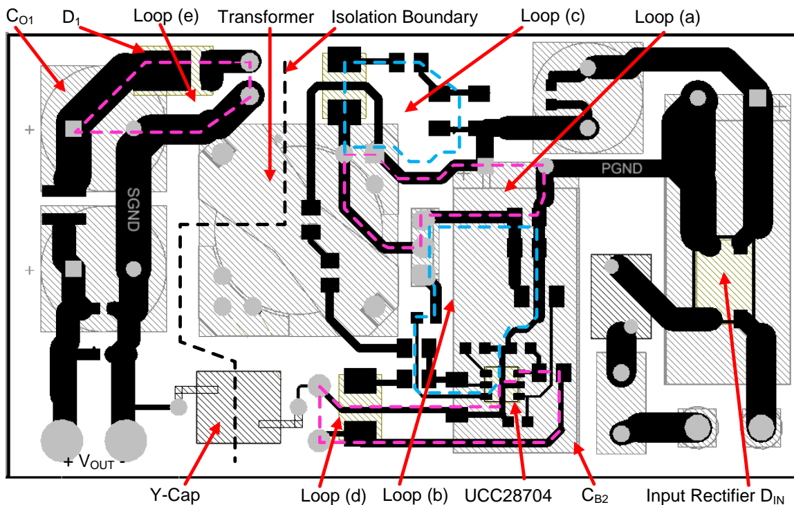
Figure 33. Layout Example
