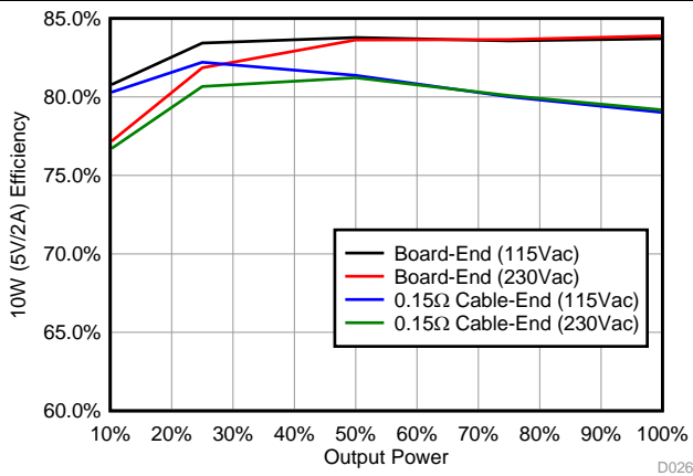
Figure 26. Efficiency
