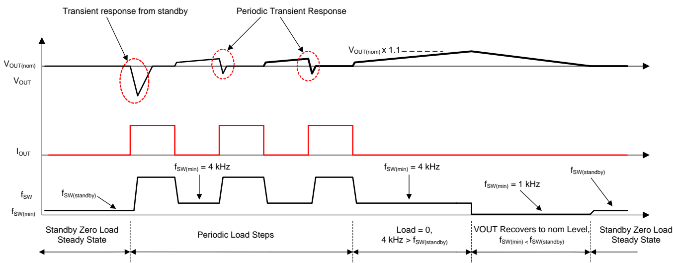
Figure 23. Dynamic Load Response
