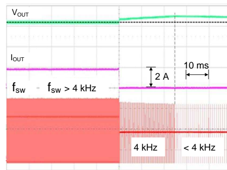
Figure 29. Response to Load Step-Down
