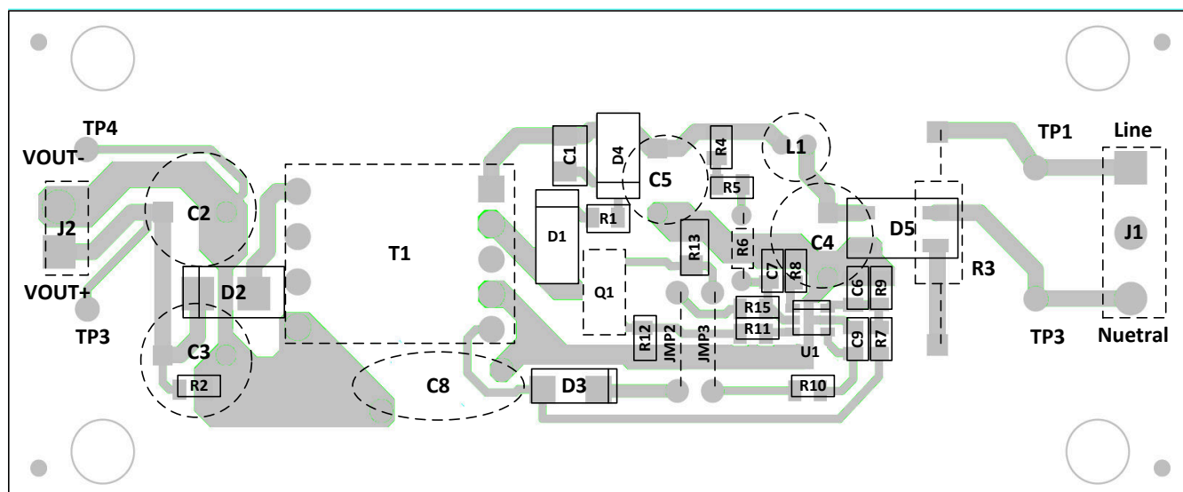
Figure 10-2. Layout Example
