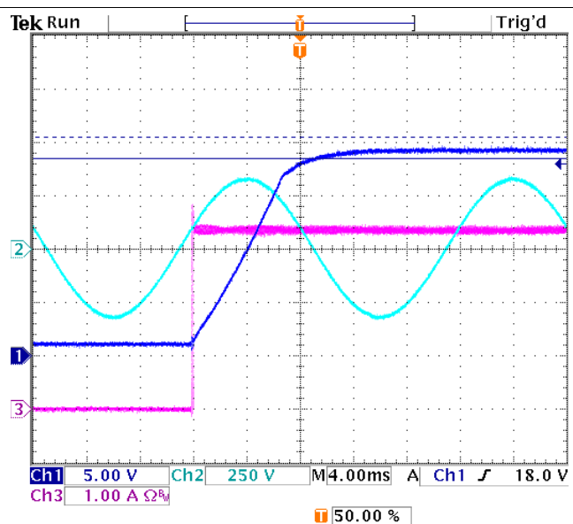
Figure 52. Output Rise-Time, 230-V AC , 3.35 A CC Load
