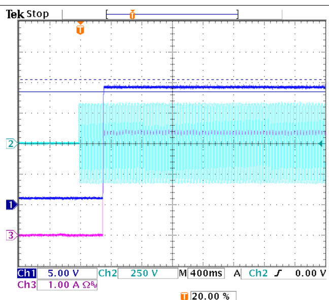
Figure 50. Start-Up from 230-V AC , 3.35-A CC Load
