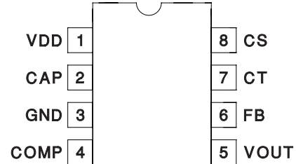
DIL-8, SOIC-8 (Top View) J or N Package, D Package
