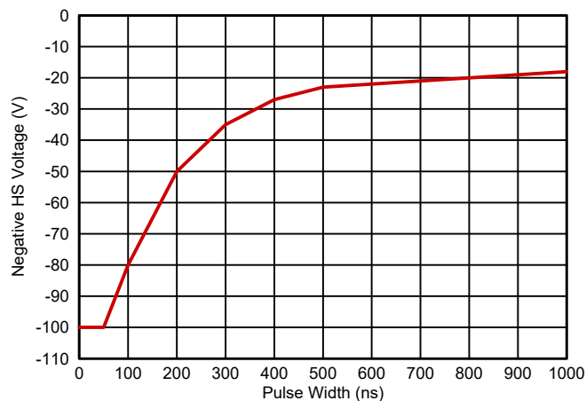
Figure 6-8. NTSOA (Negative Transient Safe Operating Area) Maximum Negative HS Voltage vs Pulse Width
