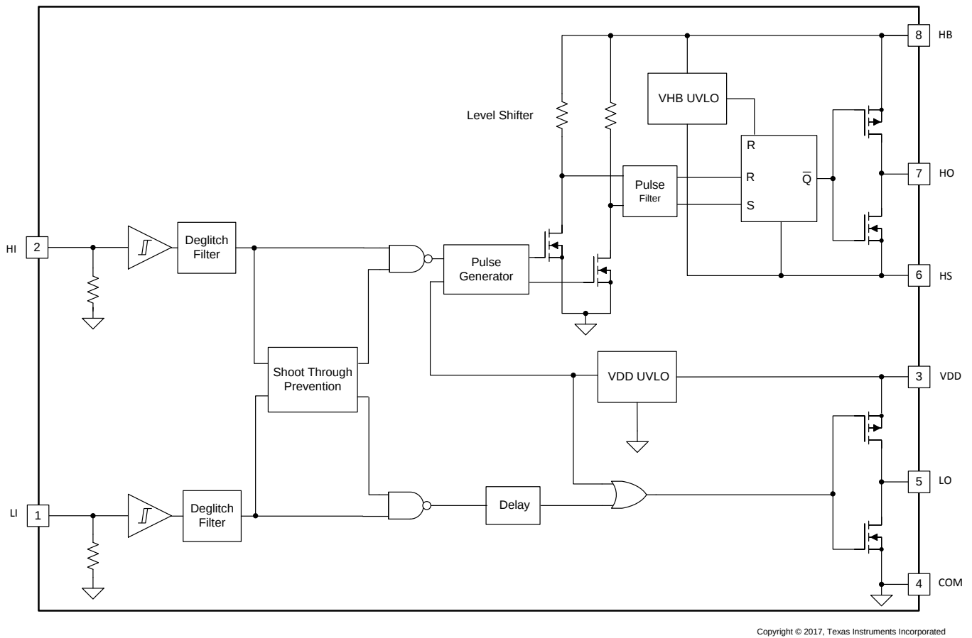
Figure 29. UCC27712-Q1 Block Diagram
