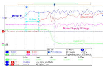
Figure 7-3. UCC27624V Used to Drive IGBT in the Boost Converter
