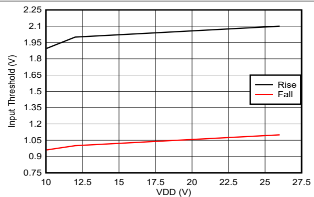
Figure 5-8. Input Thresholds
