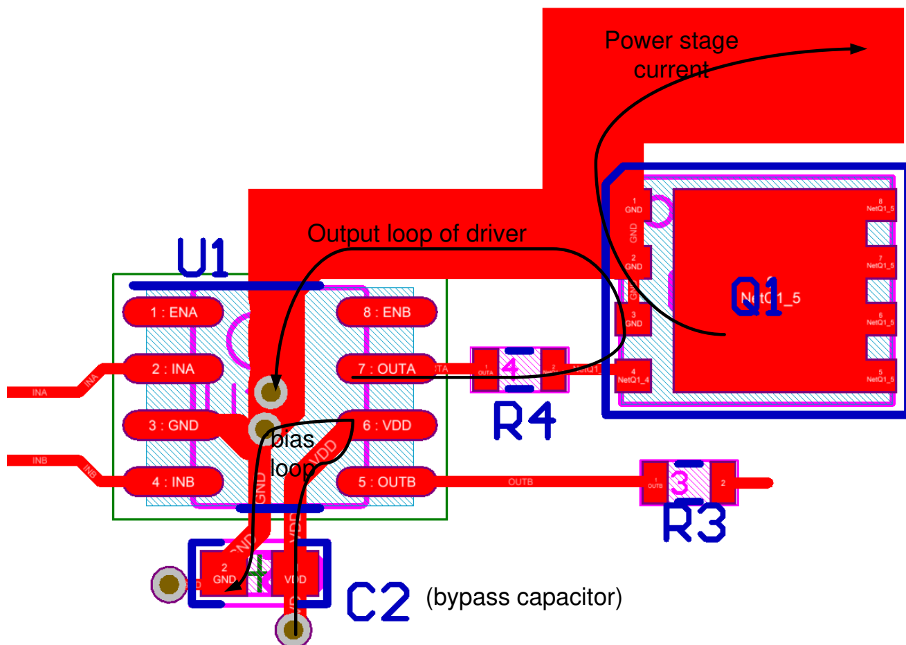
Figure 9-1. UCC27624-Q1 Layout Example
