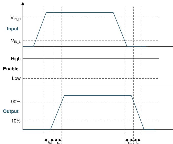
Figure 5-1. Single Input Version, IN = PWM
