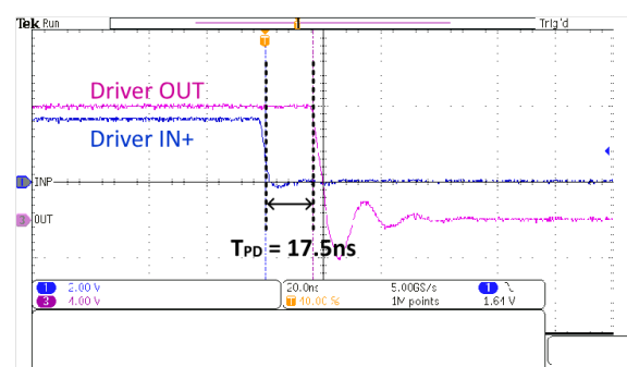
Figure 7-4. UCC27614-Q1 Falling (Turn-Off) Propagation Delay
