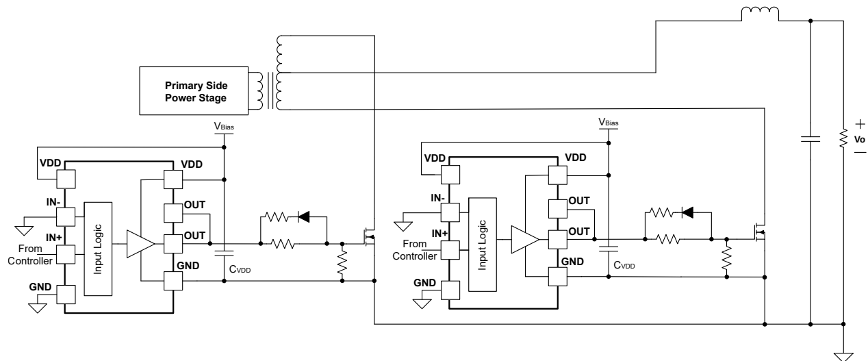
Figure 7-2. UCC27614-Q1DSG Used to Drive Secondary Side Synchronous Rectifiers
