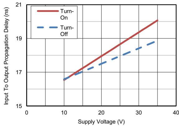
Figure 5-4. Propagation Delay vs Supply Voltage
