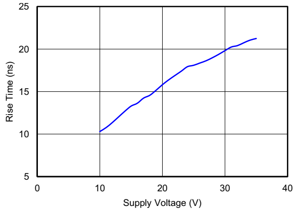
Figure 5-2. Rise Time vs Supply Voltage
