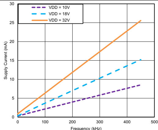
Figure 9. Operating Supply Current vs. Frequency
