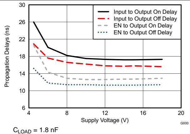
Figure 16. Propagation Delays vs Supply Voltage
