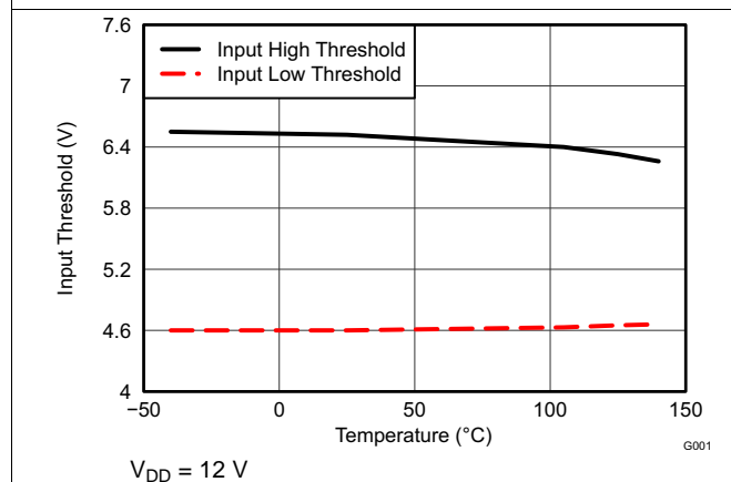
Figure 7. Input Threshold vs Temperature
