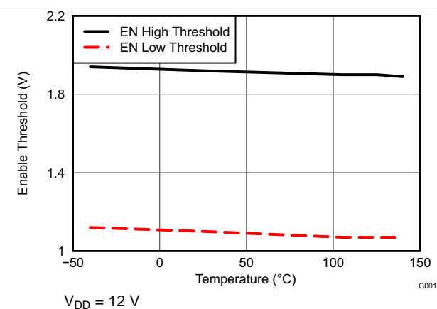
Figure 8. Enable Threshold vs Temperature
