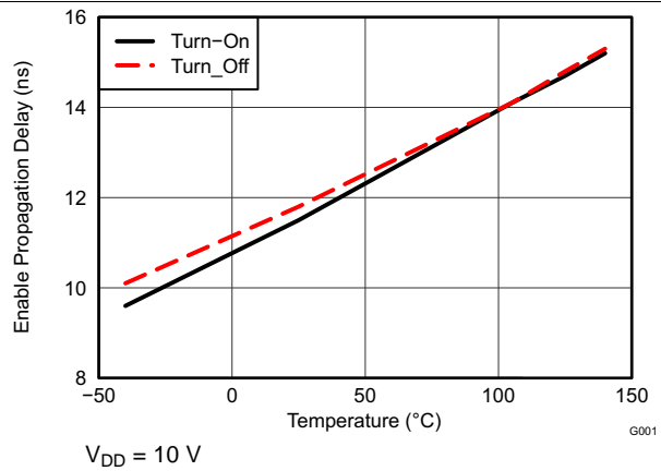
Figure 14. En To Output Propagation Delay vs Temperature
