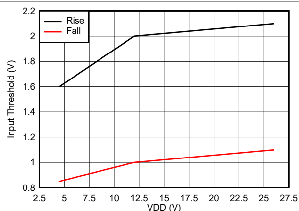
Figure 6-8. Input Thresholds
