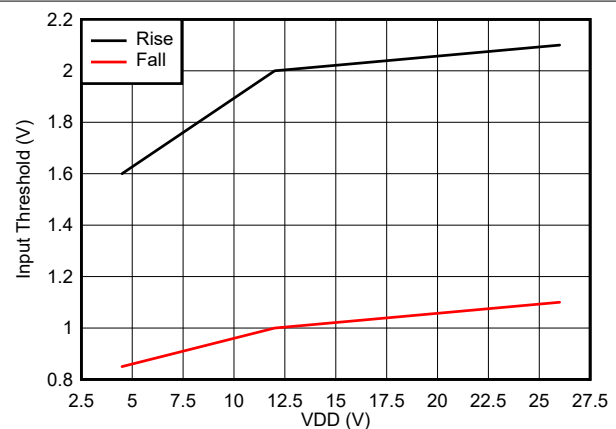
Figure 6-8. Input Thresholds
