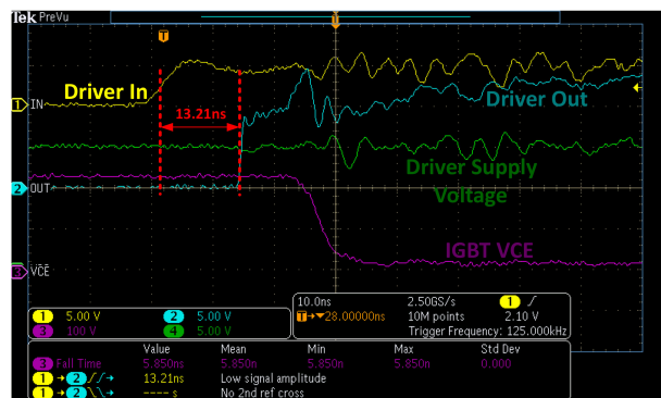
Figure 8-4. Turn-On Propagation Delay Waveform
