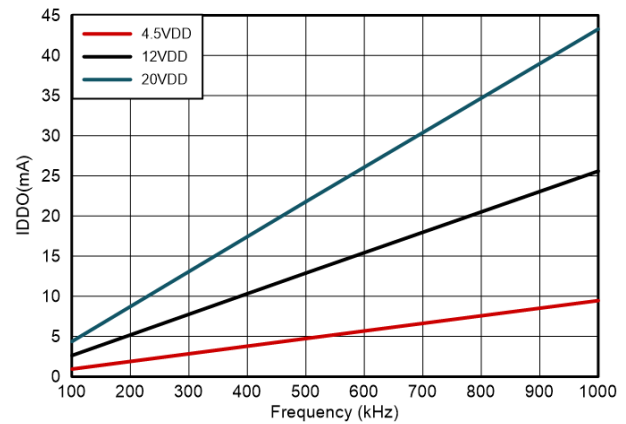
Figure 6-4. Operating Supply Current (both outputs switching)
