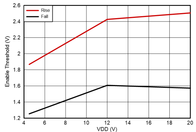
Figure 6-8. Enable Threshold
