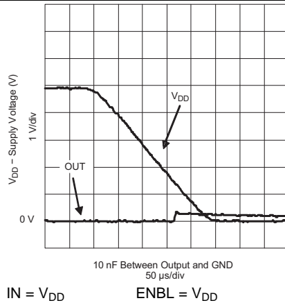
Figure 16. Output Behavior vs Supply Voltage (Inverting)
