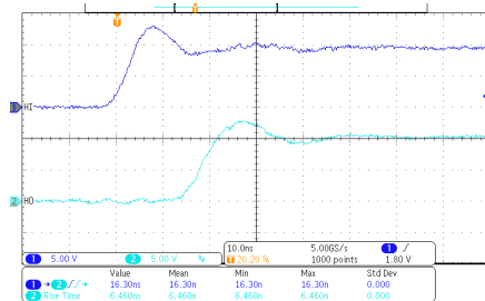
Figure 7-4. HO Rise Time and HI to HO Turn-on Propagation Delay
