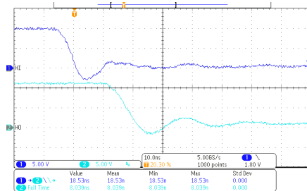
Figure 7-5. HO Fall Time and HI to HO Turn-off Propagation Delay
