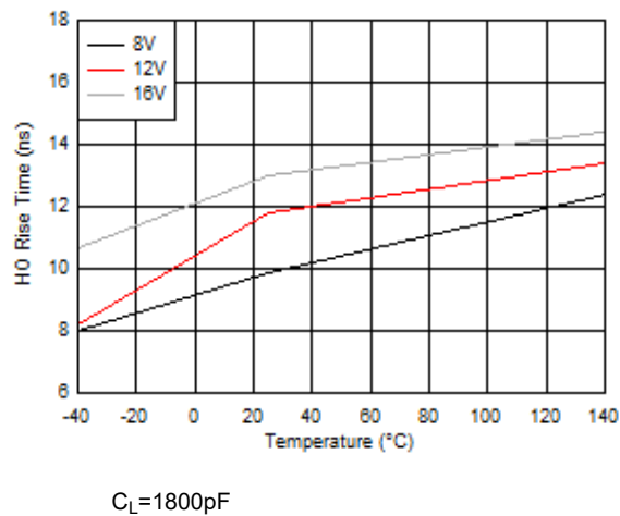
Figure 6-18. HO Rise Time
