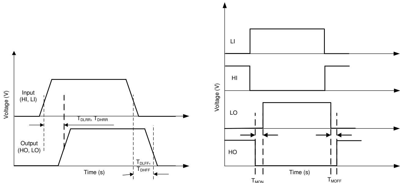
Figure 6-1. Timing Diagram
