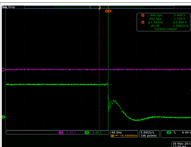
Figure 8-4. HO Fall Time
