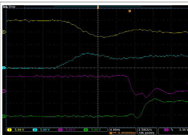
Figure 8-8. Propagation Delay and Delay Matching
