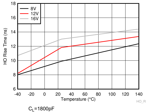
Figure 6-18. HO Rise Time
