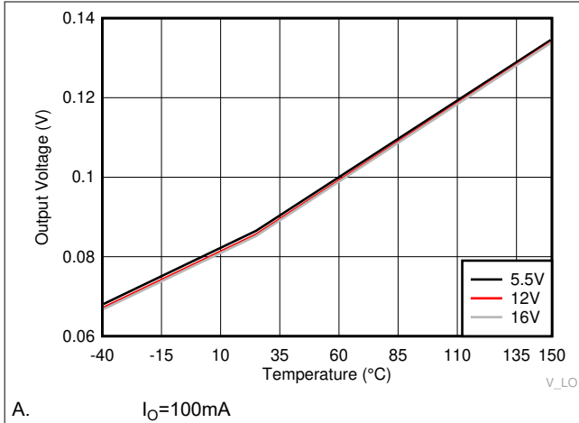
Figure 6-13. LO Low Output Voltage ( V_{LOL} )
