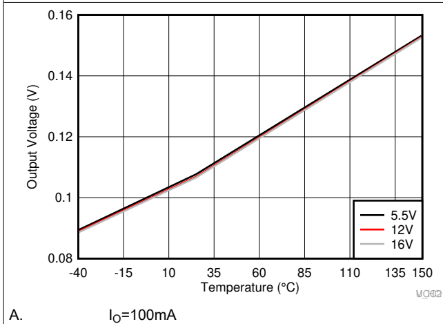
Figure 6-15. HO Low Output Voltage ( V_{HOL} )
