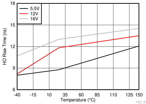
Figure 6-19. HO Rise Time
