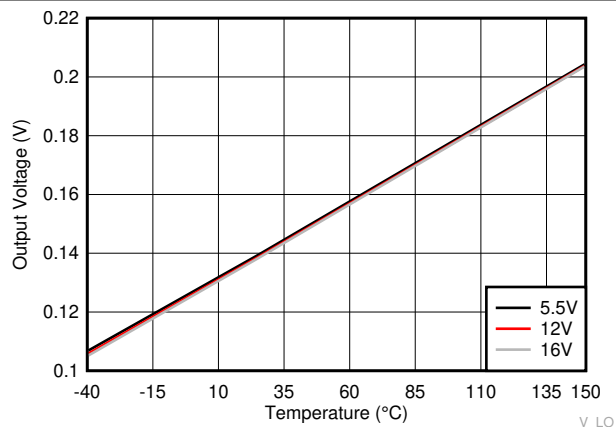
A. I_O = -100\text{mA} Figure 6-14. LO High Output Voltage ( V_{LOH} )
