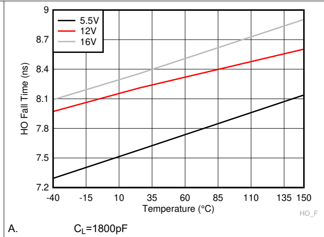
Figure 6-20. HO Fall Time
