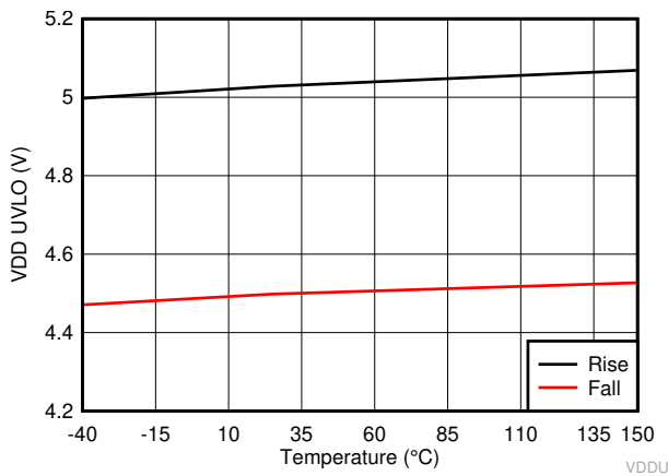
Figure 6-9. VDD UVLO Threshold
