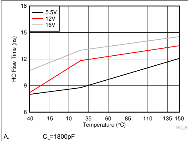
Figure 6-19. HO Rise Time
