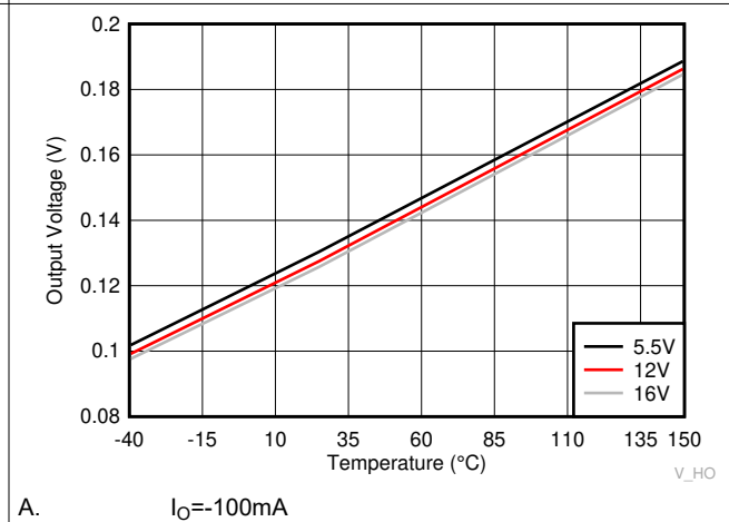
Figure 6-16. HO High Output Voltage ( V_{HOH} )
