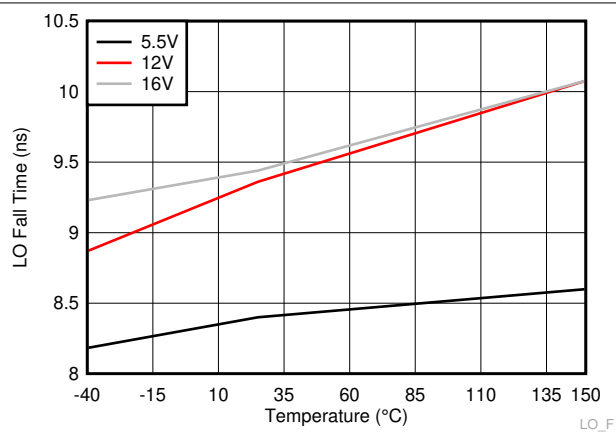
A. C_L = 1800\text{pF} Figure 6-18. LO Fall Time
