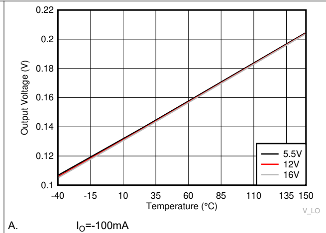
Figure 6-14. LO High Output Voltage ( V_{LOH} )
