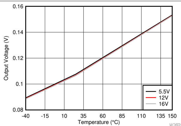
A. I_O = 100\text{mA} Figure 6-15. HO Low Output Voltage ( V_{HOL} )
