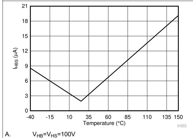
Figure 6-5. HB to VSS Quiescent Current
