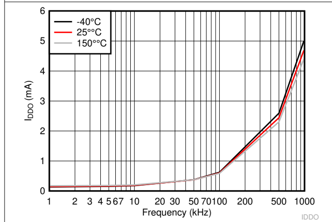
Figure 6-3. VDD Operating Current
