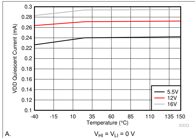
Figure 6-1. VDD Quiescent Current
