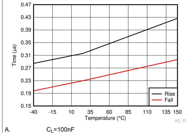
Figure 6-22. HO Rise andamp; Fall Time
