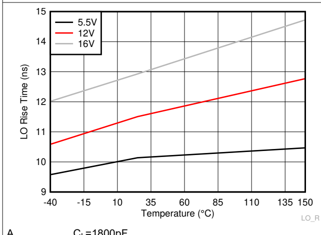
Figure 6-17. LO Rise Time
