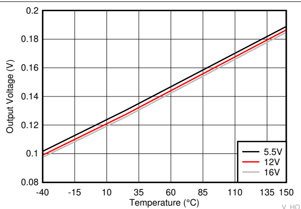
A. I_O = -100\text{mA} Figure 6-16. HO High Output Voltage ( V_{HOH} )
