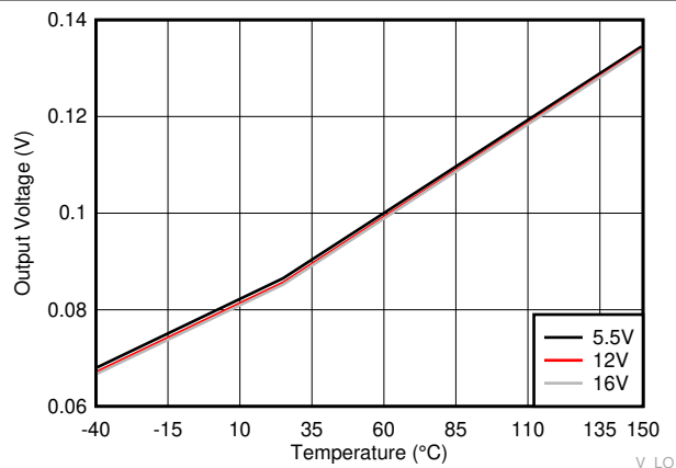
A. I_O = 100\text{mA} Figure 6-13. LO Low Output Voltage ( V_{LOL} )
