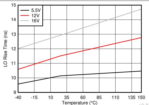
A. C_L = 1800\text{pF} Figure 6-17. LO Rise Time
