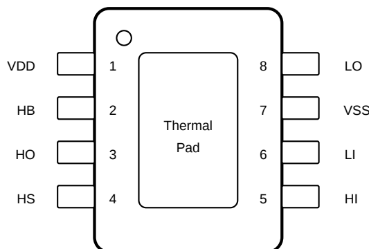
Figure 4-1. DDA Package 8-Pin SO-PowerPAD Top View
