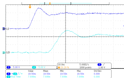
C_L = 1nF V_{DD} = 12V Figure 7-2. LO Rise Time and LI to LO Turn-on Propagation Delay
