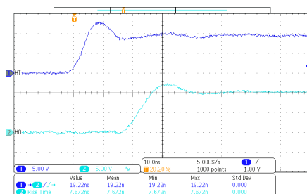
C_L = 1nF V_{DD} = 12V Figure 7-4. HO Rise Time and HI to HO Turn-on Propagation Delay
