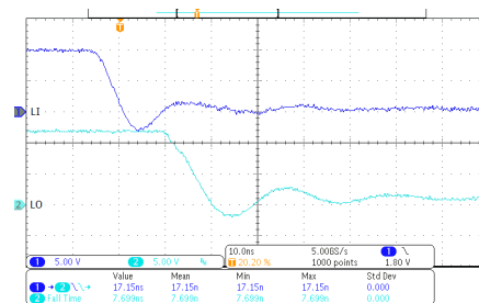
C_L = 1nF V_{DD} = 12V Figure 7-3. LO Fall Time and LI to LO Turn-off Propagation Delay
