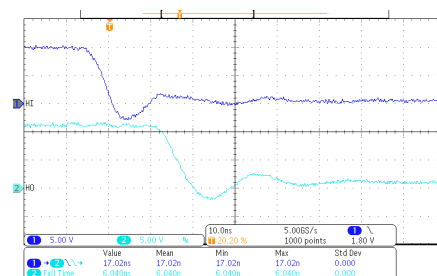
C_L = 1nF V_{DD} = 12V Figure 7-5. HO Fall Time and HI to HO Turn-off Propagation Delay
