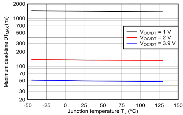
Figure 7-9. Programmed maximum dead-time vs junction temperature
