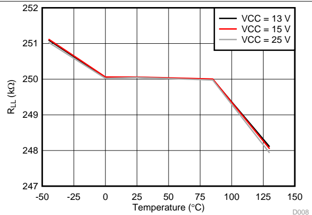
Figure 8. R_{LL} vs Temperature
