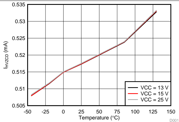
Figure 19. I_{HVZCD} vs Temperature
