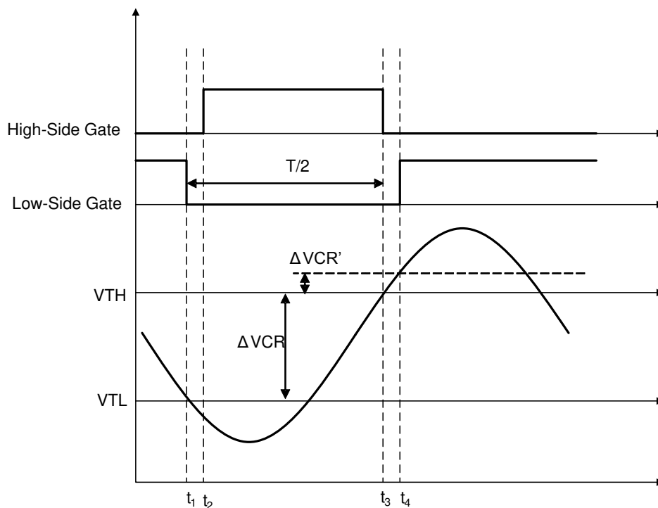
Figure 29. HHC Gate On/Off Control Principle
