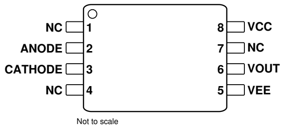
Figure 5-4. UCC23514V DWV Package 8-pin SOIC-WB Top View
