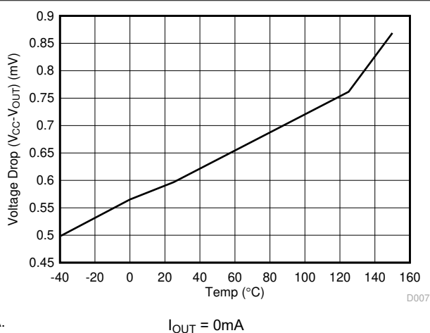
Figure 6-8. V_{OH} (No Load) versus Temperature
