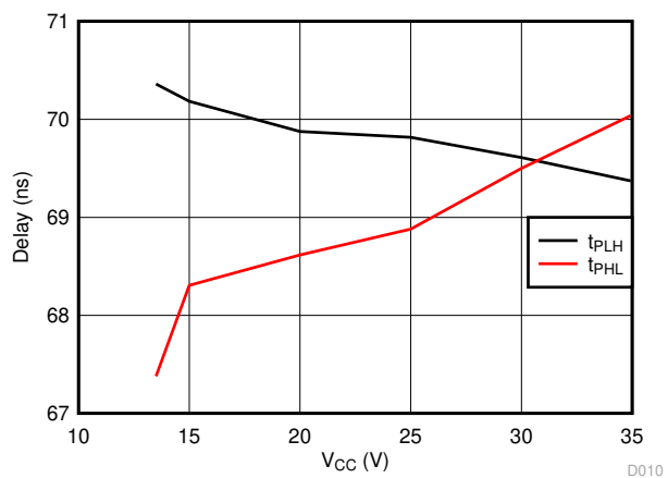
Figure 6-11. Propagation delay versus Supply voltage
