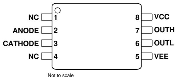
Figure 5-3. UCC23514S DWV Package 8-pin SOIC-WB Top View
