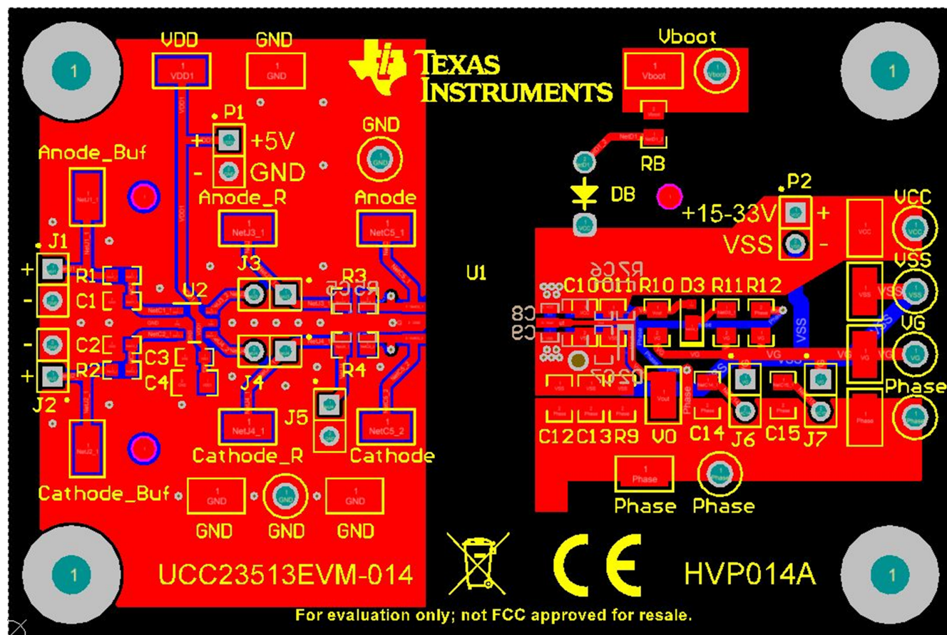
Figure 12-1. Layout Example
