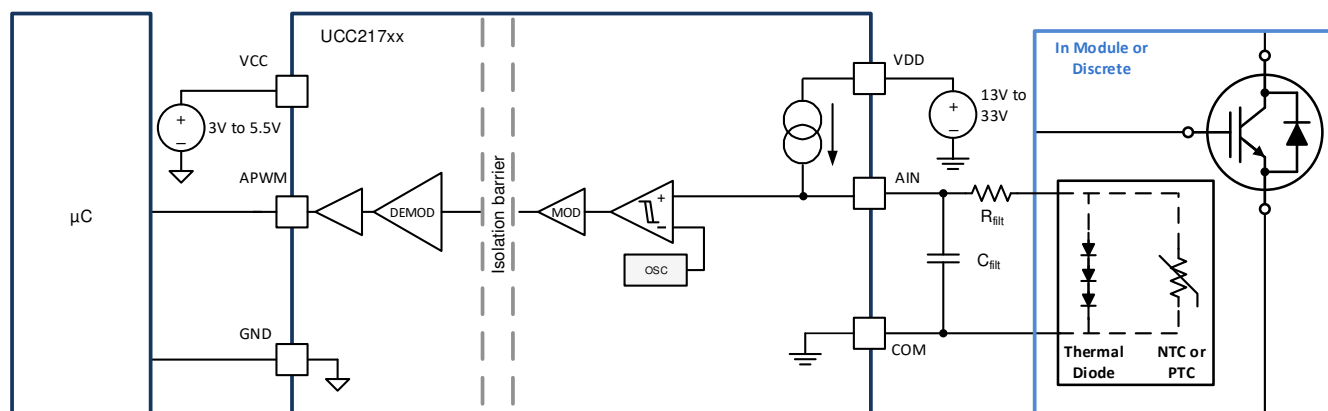
Figure 8-7. Thermal Diode or Thermistor Temperature Sensing Configuration
