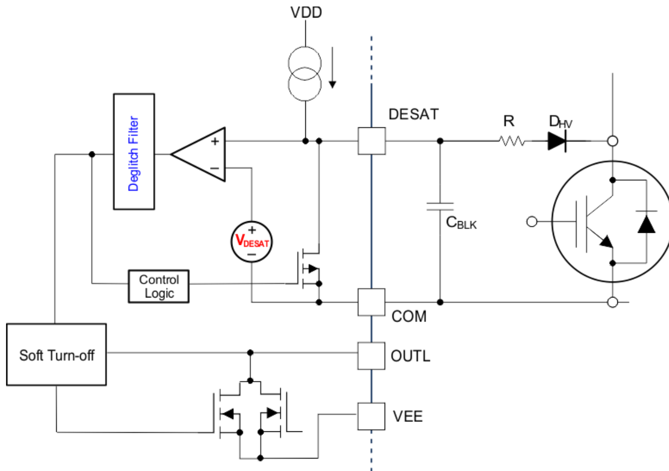
Figure 7-6. Soft Turn-off
