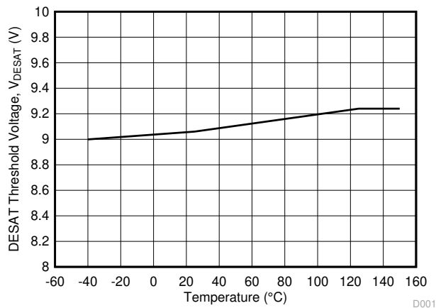
Figure 5-23. V_{DESAT} DESAT Threshold Voltage vs Temperature
