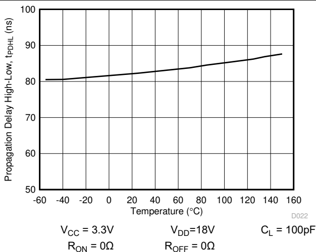
Figure 5-15. Propagation Delay t_{PDHL} vs. Temperature
