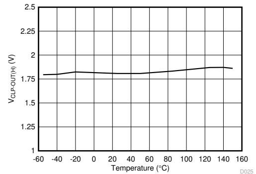
Figure 6-19. V_{CLP-OUT(H)} Short Circuit Clamping Voltage vs. Temperature
