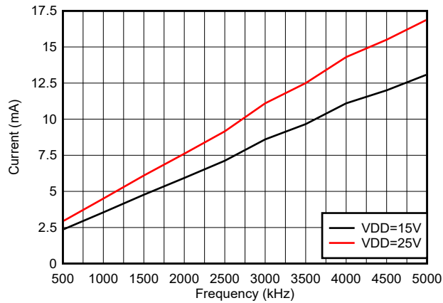
Figure 5-4. Per Channel Current Consumption vs Frequency
