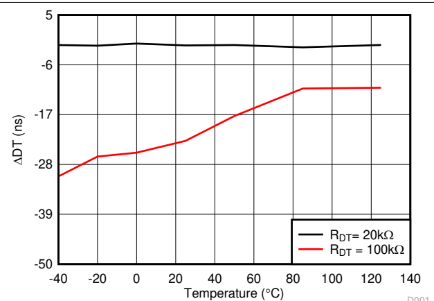
Figure 5-27. Dead Time Matching vs Temperature
