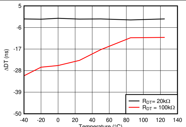
Figure 5-25. Dead Time Matching vs Temperature
