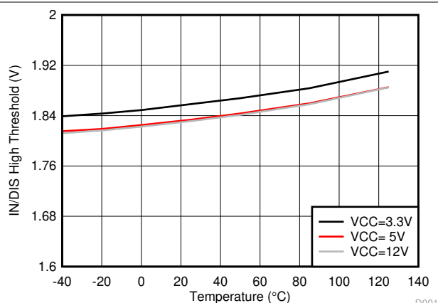
Figure 5-23. INA/B/EN High Threshold
