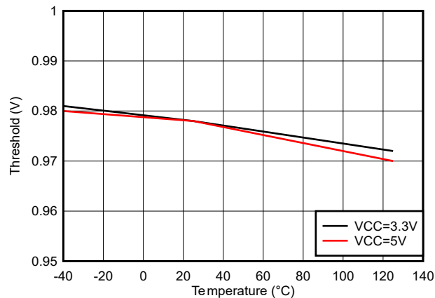
Figure 5-24. IN/DIS Low Threshold
