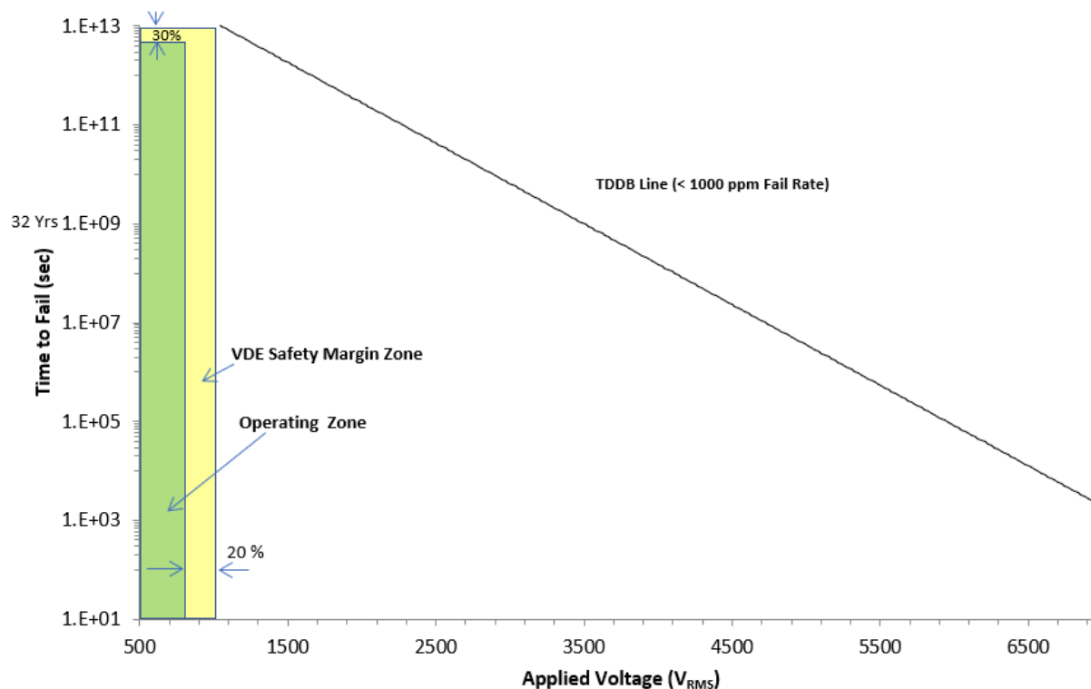
Figure 5-3. Basic Isolation Capacitor Life Time Projection
