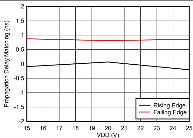
Figure 5-14. Propagation Delay Matching ( t_{\text{DM}} ) vs VDD
