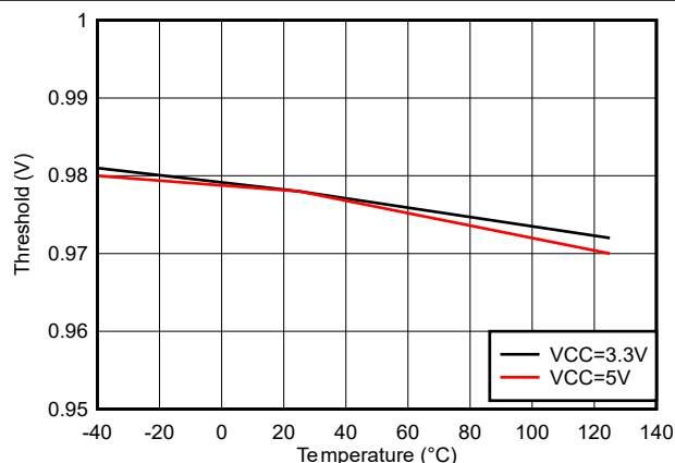
Figure 5-20. IN/DIS Low Threshold
