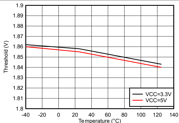
Figure 5-21. IN/DIS High Threshold
