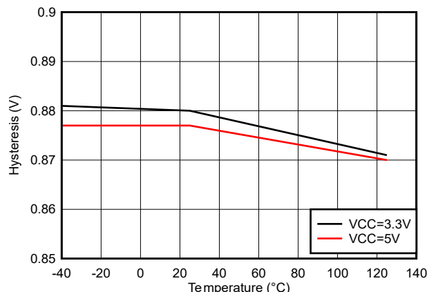
Figure 5-19. IN/DIS Hysteresis vs Temperature
