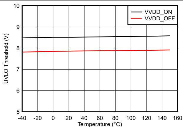
Figure 5-17. VDD 8-V UVLO Threshold vs Temperature
