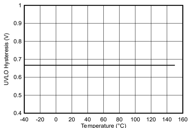
Figure 5-18. VDD 8-V UVLO Hysteresis vs Temperature
