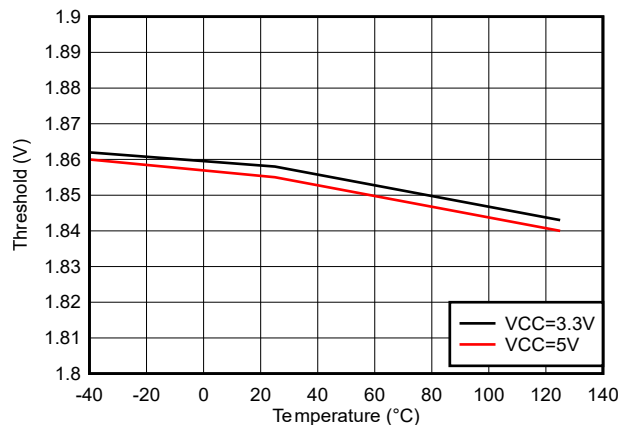
Figure 6-11. INA/INB/DIS High Threshold Voltage
