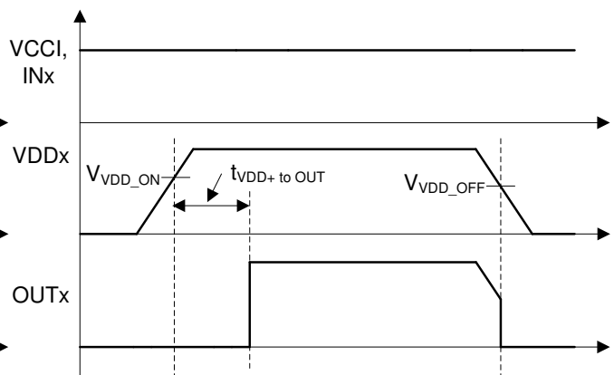
Figure 7-7. VDDA/B Power-up UVLO Delay
