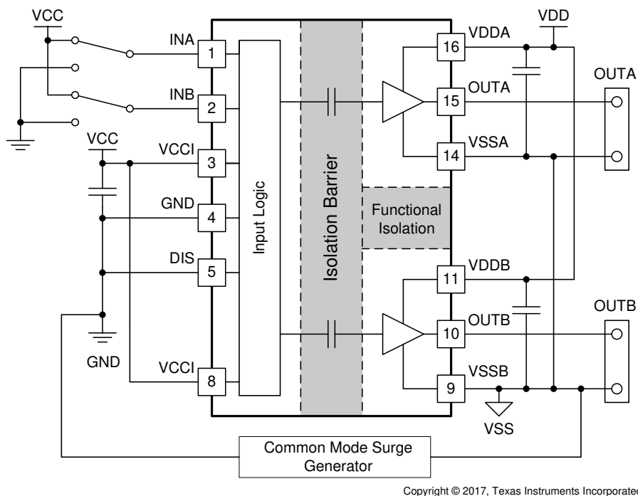
Figure 7-8. Simplified CMTI Testing Setup
