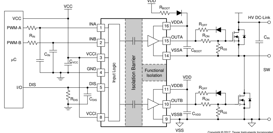
Typical Application
