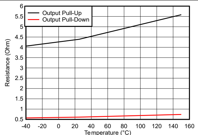
Figure 6-14. OUT Pullup and Pulldown Resistance
