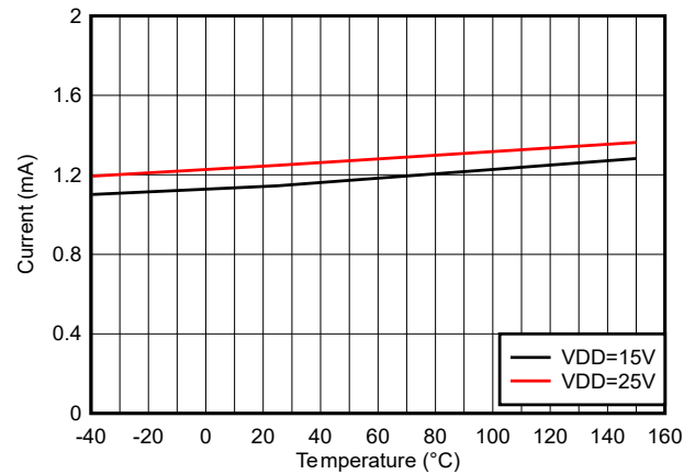
Figure 6-4. VDD Per Channel Quiescent Current ( I_{VDDA} , I_{VDDB} )
