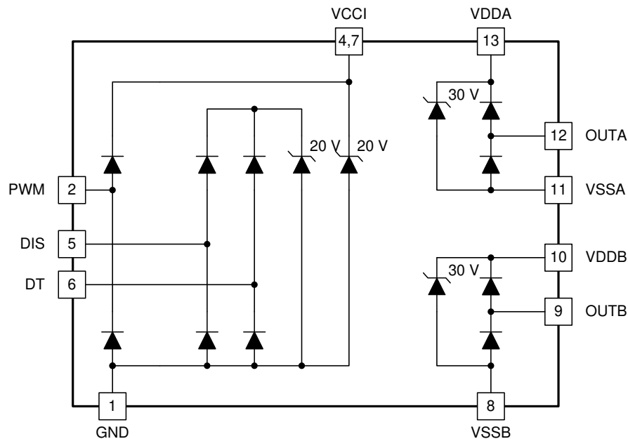
Figure 35. ESD Structure
