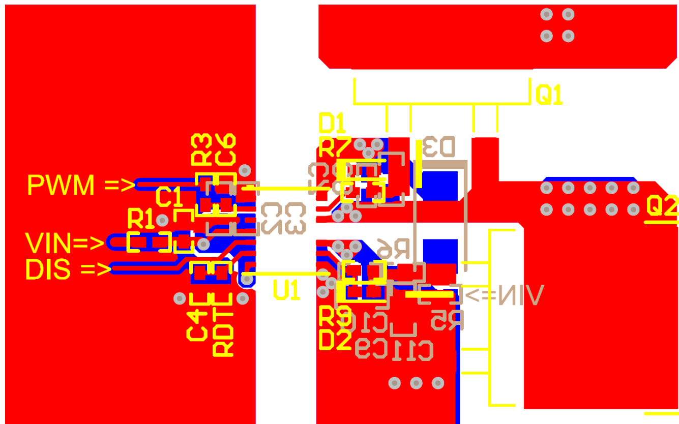
Figure 43. Layout Example
