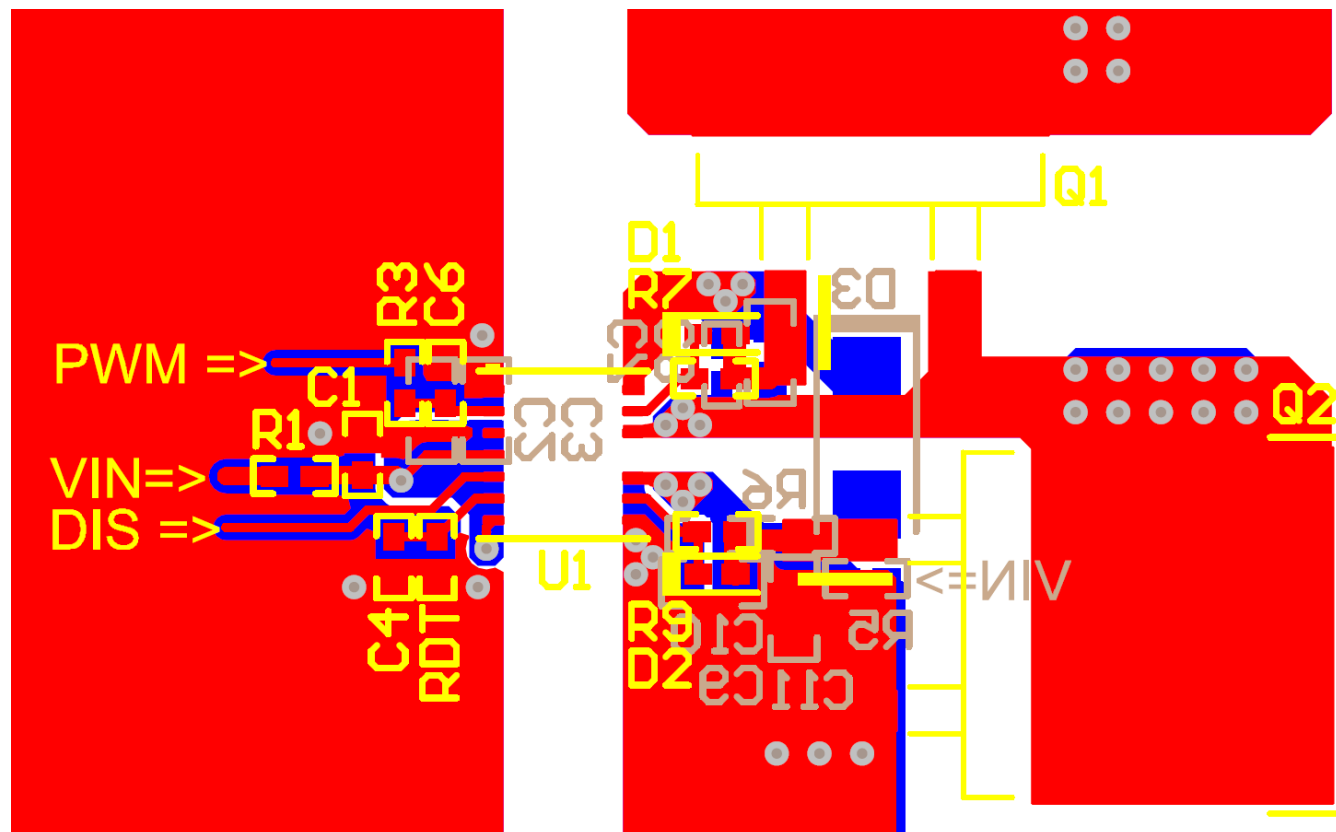
Figure 41. Layout Example
