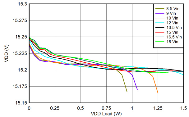
Figure 6-29. UCC14341B-Q1 V_{DD-VEE} Load Regulation: T_{AMBIENT} = 85^{\circ}C , V_{DD-VEE} = 15V , V_{COM-VEE} = 4V
