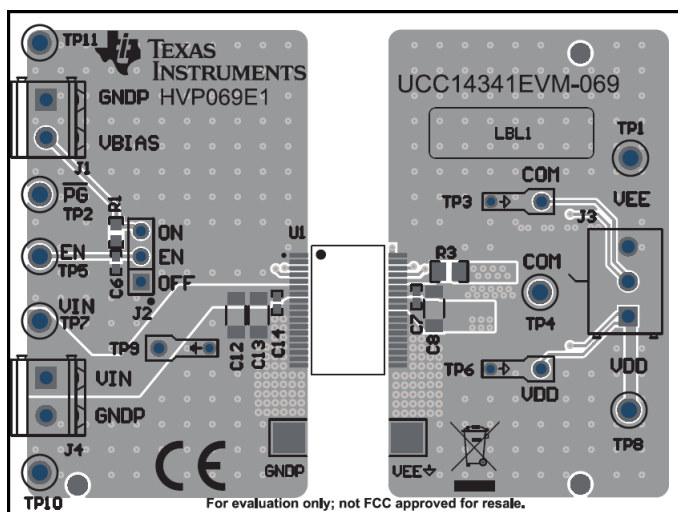
Figure 8-21. UCC14341-Q1EVM, PCB Top Layer, Assembly
