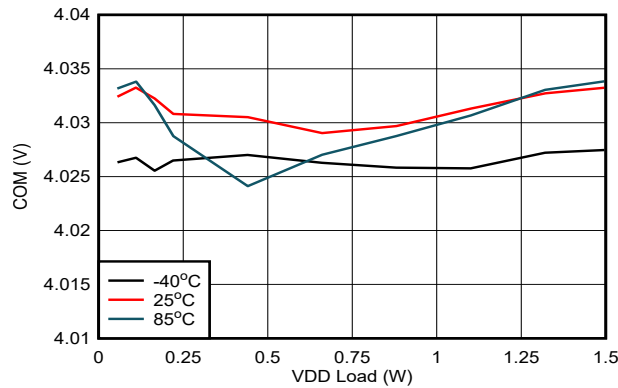
Figure 6-16. V_{COM-VEE} Load Regulation: V_{IN} = 16.5V , V_{DD-VEE} = 22V , V_{COM-VEE} = 4V
