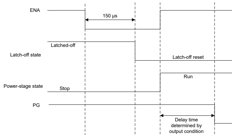
Figure 7-6. Latch-Off Reset Using ENA Pin
