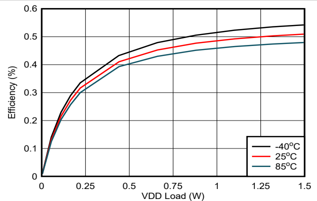
Figure 6-19. Efficiency vs. Load on V_{DD-VEE} : V_{IN} = 15V , V_{DD-VEE} = 22V , V_{COM-VEE} = 4V , No Load on V_{COM-VEE}
