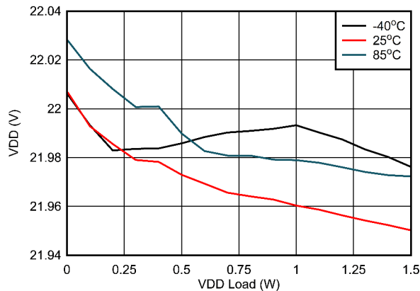
Figure 6-10. V_{D\overline{D}-VEE} Load Regulation: V_{IN} = 13.5V , V_{D\overline{D}-VEE} = 22V , V_{COM-VEE} = 4V
