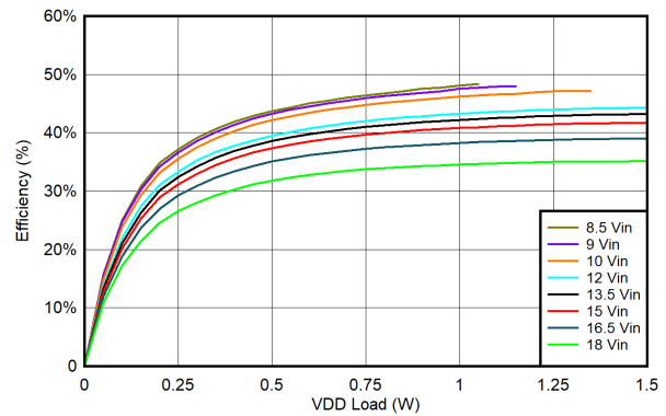
Figure 6-31. UCC14341B-Q1 Efficiency vs. Load on V_{DD-VEE} : T_{AMBIENT} = 25^{\circ}C , V_{DD-VEE} = 15V , V_{COM-VEE} = 4V , No Load on V_{COM-VEE}
