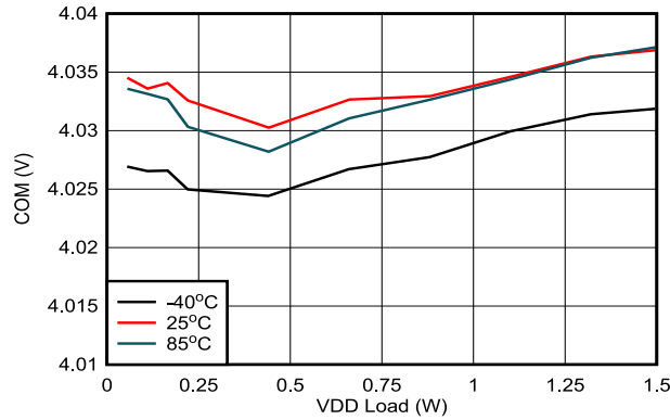
Figure 6-14. V_{COM-VEE} Load Regulation: V_{IN} = 13.5V , V_{DD-VEE} = 22V , V_{COM-VEE} = 4V
