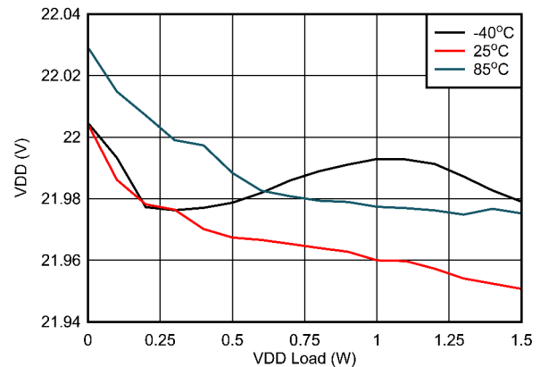
Figure 6-11. V_{D\overline{D}-VEE} Load Regulation: V_{IN} = 15V , V_{D\overline{D}-VEE} = 22V , V_{COM-VEE} = 4V
