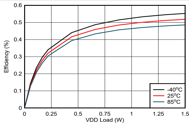
Figure 6-18. Efficiency vs. Load on V_{DD-VEE} : V_{IN} = 13.5V , V_{DD-VEE} = 22V , V_{COM-VEE} = 4V , No Load on V_{COM-VEE}
