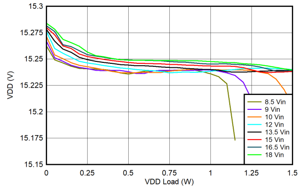
Figure 6-27. UCC14341B-Q1 V_{DD-VEE} Load Regulation: T_{AMBIENT} = -40^{\circ}C , V_{DD-VEE} = 15V , V_{COM-VEE} = 4V
