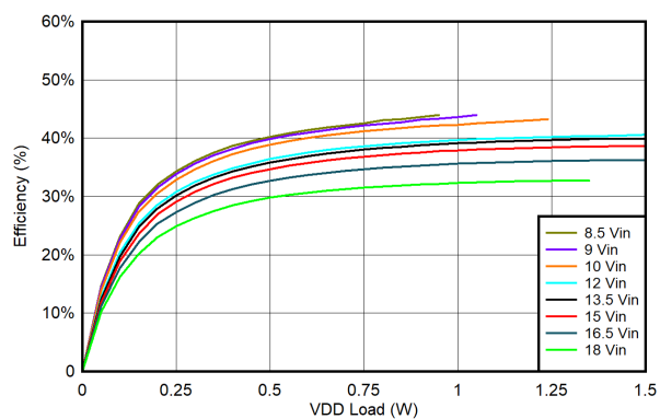
Figure 6-32. UCC14341B-Q1 Efficiency vs. Load on V_{DD-VEE} : T_{AMBIENT} = 85^{\circ}\text{C} , V_{DD-VEE} = 15\text{V} , V_{COM-VEE} = 4\text{V} , No Load on V_{COM-VEE}
