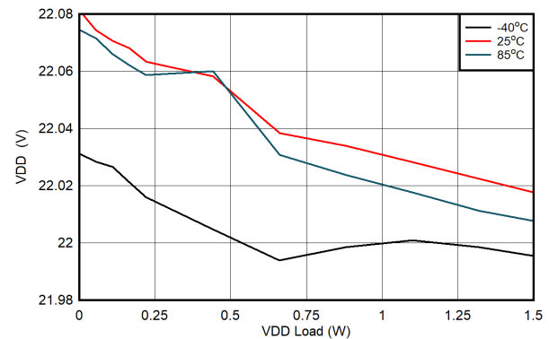
Figure 6-13. V_{D\overline{D}-VEE} Load Regulation: V_{IN} = 18V , V_{D\overline{D}-VEE} = 22V , V_{COM-VEE} = 4V
