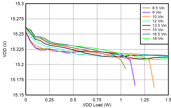
Figure 6-28. UCC14341B-Q1 V_{DD-VEE} Load Regulation: T_{AMBIENT} = 25^{\circ}C , V_{DD-VEE} = 15V , V_{COM-VEE} = 4V
