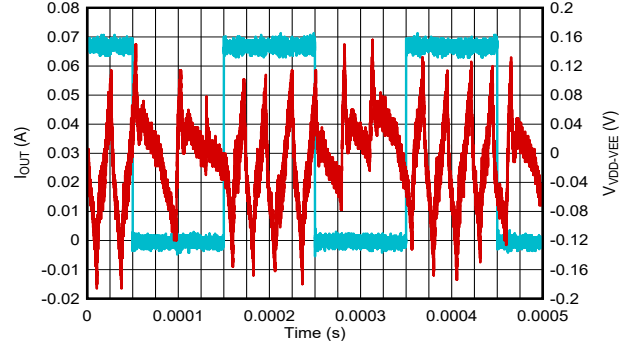
Figure 6-9. Load Transient Response: Between No Load and 1.5W, V_{IN} = 15V , V_{D\overline{D}-VEE} = 22V , V_{COM-VEE} = 4V
