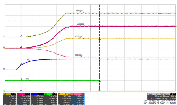
Figure 6-7. Start-up: V_{IN} = 15\text{V} , V_{DD-VEE} = 22\text{V} , V_{COM-VEE} = 4\text{V} , I_{VDD-VEE} = 68\text{mA} , No Load on V_{COM-VEE} . Time Scale: 1ms/div.
