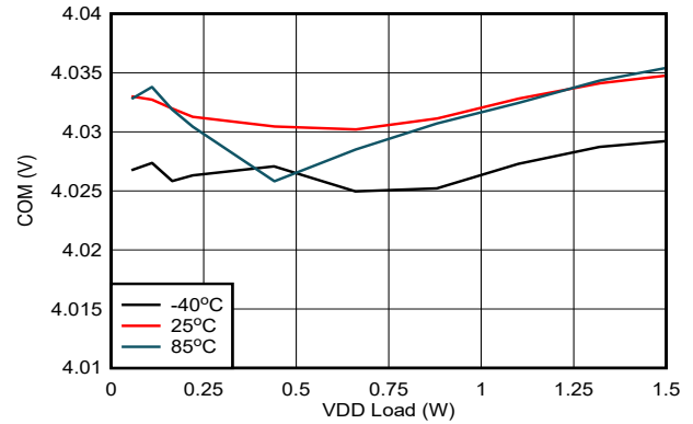
Figure 6-15. V_{COM-VEE} Load Regulation: V_{IN} = 15V , V_{DD-VEE} = 22V , V_{COM-VEE} = 4V
