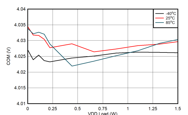
Figure 6-17. V_{COM-VEE} Load Regulation: V_{IN} = 18V , V_{DD-VEE} = 22V , V_{COM-VEE} = 4V
