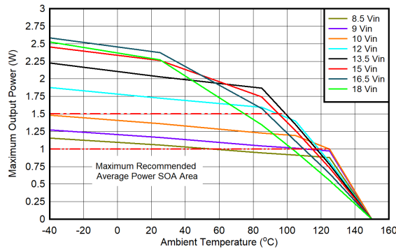
Figure 6-26. UCC14341B-Q1 SOA Derating Curves: V_{DD-VEE} = 15V , V_{COM-VEE} = 5V , T_{shut} = 160^{\circ}C , No Load on V_{COM-VEE}
