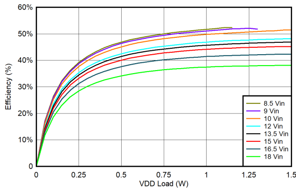
Figure 6-30. UCC14341B-Q1 Efficiency vs. Load on V_{DD-VEE} : T_{AMBIENT} = -40^{\circ}C , V_{DD-VEE} = 15V , V_{COM-VEE} = 4V , No Load on V_{COM-VEE}
