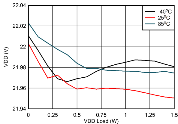
Figure 6-12. V_{D\overline{D}-VEE} Load Regulation: V_{IN} = 16.5V , V_{D\overline{D}-VEE} = 22V , V_{COM-VEE} = 4V
