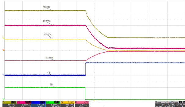
Figure 6-8. Shutdown: V_{IN} = 15V , V_{D\overline{D}-VEE} = 22V , V_{COM-VEE} = 4V , I_{D\overline{D}-VEE} = 68mA , No Load on V_{COM-VEE} . Time Scale: 2ms/div.
