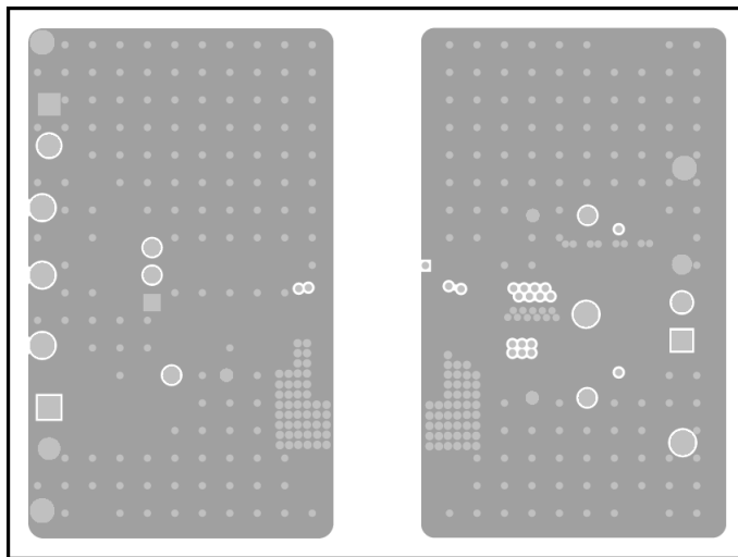
Figure 8-22. UCC14341-Q1EVM, Signal Layer 2 (Same as Layer 3)
