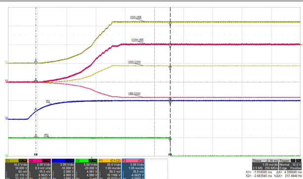
Figure 7-6. Start-up: V_{IN} = 15\text{ V} , V_{D\bar{D}-VEE} = 22\text{ V} , V_{COM-VEE} = 4\text{ V} , I_{D\bar{D}-VEE} = 68\text{ mA} , No Load on V_{COM-VEE} . Time Scale: 1ms/div.
