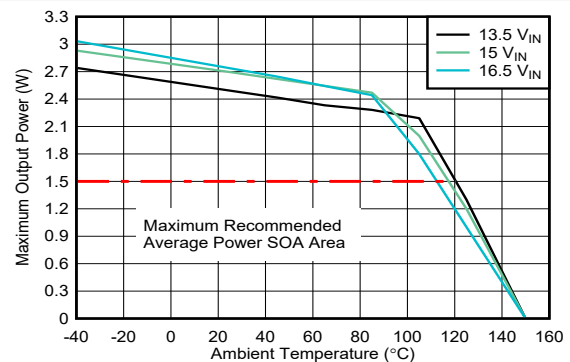
Figure 7-2. SOA Derating Curves: V_{D\bar{D}-VEE} = 18\text{ V} , V_{COM-VEE} = 3\text{ V} , T_{shut}=160^\circ\text{C} , No Load on V_{COM-VEE}
