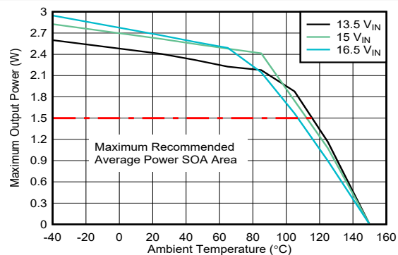
Figure 7-1. SOA Derating Curves: V_{D\bar{D}-VEE} = 15\text{ V} , V_{COM-VEE} = 5\text{ V} , T_{shut}=160^\circ\text{C} , No Load on V_{COM-VEE}
