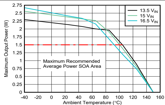
Figure 7-3. SOA Derating Curves: V_{D\bar{D}-VEE} = 22\text{ V} , V_{COM-VEE} = 4\text{ V} , T_{shut}=160^\circ\text{C} , No Load on V_{COM-VEE}
