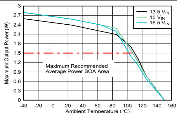
Figure 7-5. SOA Derating Curves: V_{D\bar{D}-VEE} = 22\text{ V} , V_{COM-VEE} = 4\text{ V} , T_{shut}=150^\circ\text{C} , No Load on V_{COM-VEE} , tested in a shielded box.
