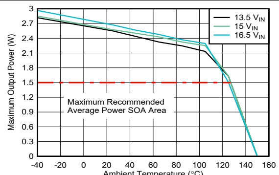
Figure 7-4. SOA Derating Curves: V_{D\bar{D}-VEE} = 25\text{ V} , V_{COM-VEE} = 5\text{ V} , T_{shut}=160^\circ\text{C} , No Load on V_{COM-VEE}
