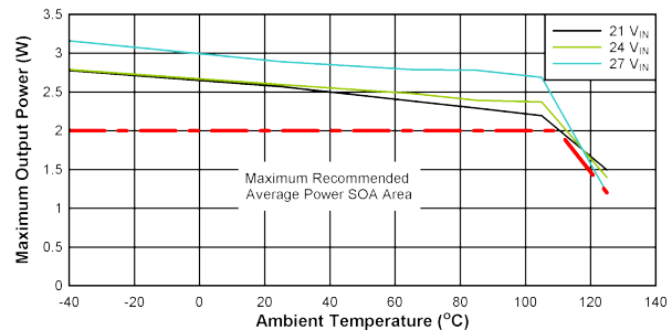
Figure 10-4. SOA Derating Curves: V_{DD-VEE} = 25\text{ V} , V_{COM-VEE} = 5\text{ V} , T_{shut}=150^\circ\text{C} , No Load on V_{COM-VEE} .
