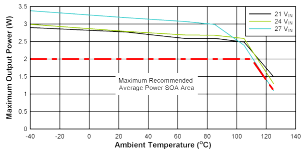
Figure 10-3. SOA Derating Curves: V_{DD-VEE} = 22\text{ V} , V_{COM-VEE} = 4\text{ V} , T_{shut}=150^\circ\text{C} , No Load on V_{COM-VEE} .
