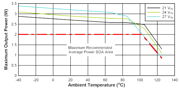
Figure 10-2. SOA Derating Curves: V_{DD-VEE} = 18\text{ V} , V_{COM-VEE} = 5\text{ V} , T_{shut}=150^\circ\text{C} , No Load on V_{COM-VEE} .
