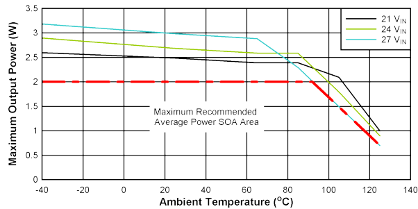
Figure 10-1. SOA Derating Curves: V_{DD-VEE} = 15\text{ V} , V_{COM-VEE} = 5\text{ V} , T_{shut}=150^\circ\text{C} , No Load on V_{COM-VEE} .
