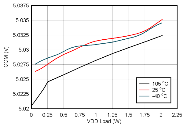
Figure 6-12. VCOM-VEE Load Regulation: VIN = 21 V, VDD-VEE = 25 V, VCOM-VEE = 5 V
