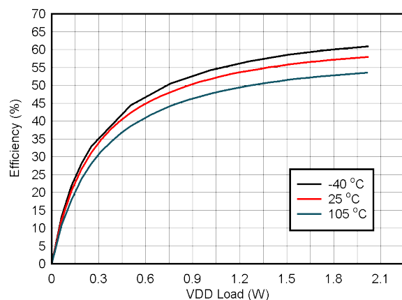
Figure 6-15. Efficiency vs Load on V_{DDE-VEE} : V_{IN} = 21\text{ V} , V_{DDE-VEE} = 25\text{ V} , V_{COM-VEE} = 5\text{ V} , No Load on V_{COM-VEE}
