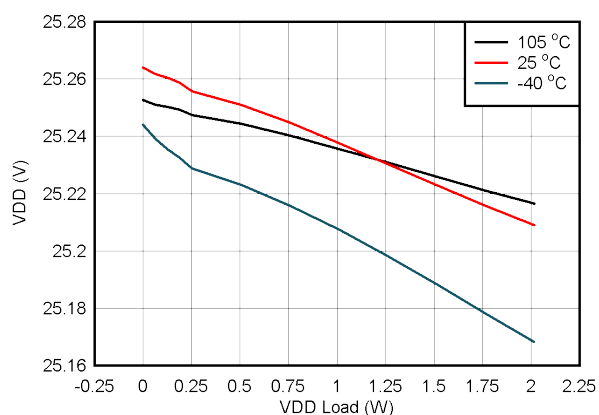
Figure 6-10. VDD-VEE Load Regulation: VIN = 24 V, VDD-VEE = 25 V, VCOM-VEE = 5 V
