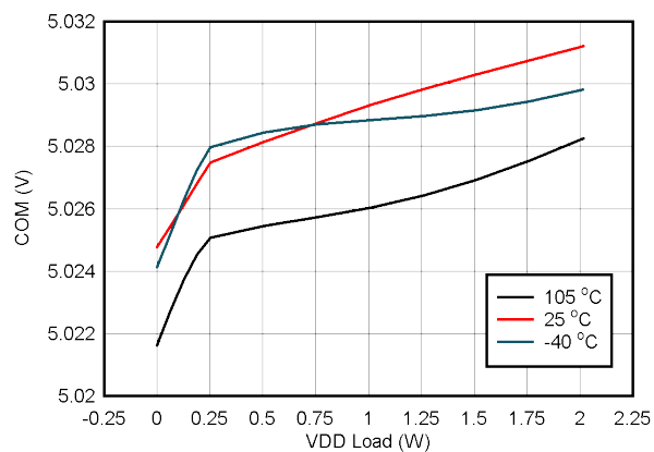
Figure 6-14. V_{COM-VEE} Load Regulation: V_{IN} = 27\text{ V} , V_{DDE-VEE} = 25\text{ V} , V_{COM-VEE} = 5\text{ V}
