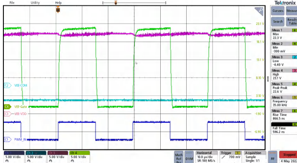
Figure 8-10. Gate Waveform Switching 100 nF at 35kHz.
