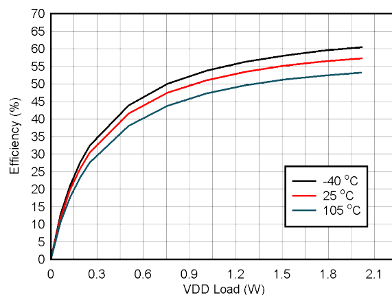
Figure 6-16. Efficiency vs Load on V_{DDE-VEE} : V_{IN} = 24\text{ V} , V_{DDE-VEE} = 25\text{ V} , V_{COM-VEE} = 5\text{ V} , No Load on V_{COM-VEE}
