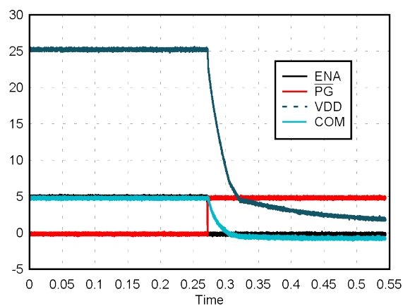
Figure 6-6. Shutdown: V_{IN} = 24\text{ V} , V_{DD-VEE} = 25\text{ V} , V_{COM-VEE} = 5\text{ V} , No Load
