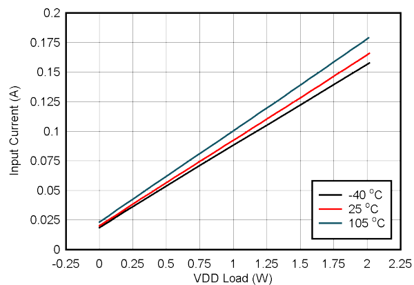
Figure 6-18. Input Current vs Load on V_{DDE-VEE} : V_{IN} = 21\text{ V} , V_{DDE-VEE} = 25\text{ V} , V_{COM-VEE} = 5\text{ V} , No Load on V_{COM-VEE}
