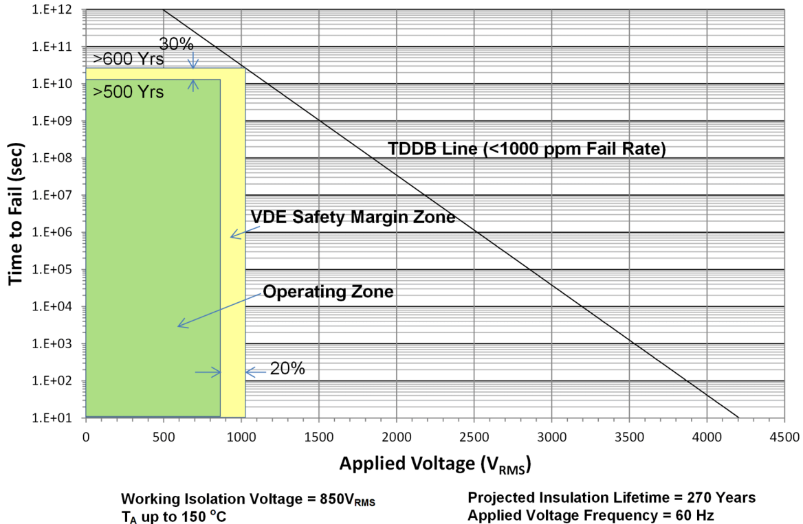
Figure 6-1. TDDB: Insulation Lifetime Projection for 850 Vrms Working Voltage.
