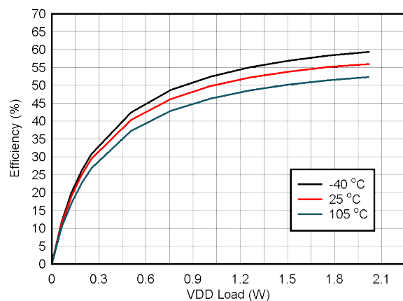
Figure 6-17. Efficiency vs Load on V_{DDE-VEE} : V_{IN} = 27\text{ V} , V_{DDE-VEE} = 25\text{ V} , V_{COM-VEE} = 5\text{ V} , No Load on V_{COM-VEE}
