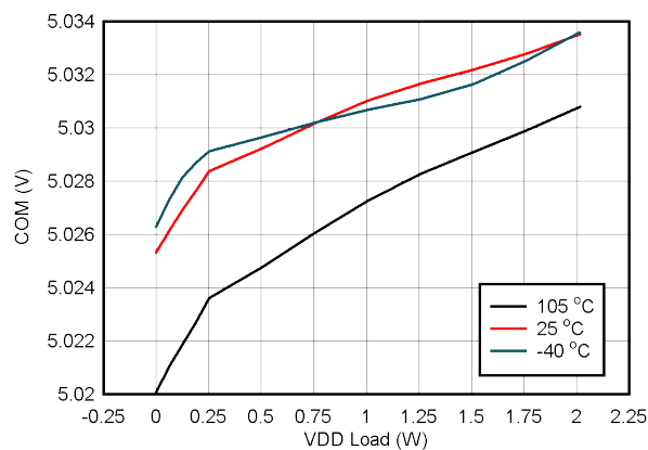
Figure 6-13. V_{COM-VEE} Load Regulation: V_{IN} = 24\text{ V} , V_{DDE-VEE} = 25\text{ V} , V_{COM-VEE} = 5\text{ V}
