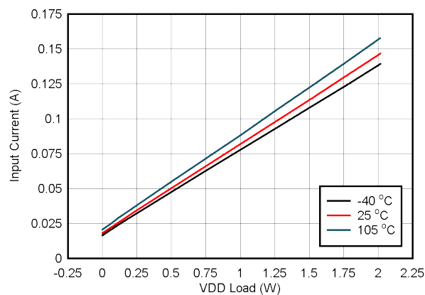
Figure 6-19. Input Current vs Load on V_{DD-VEE} : V_{IN} = 24 V, V_{DD-VEE} = 25 V, V_{COM-VEE} = 5 V, No Load on V_{COM-VEE}
