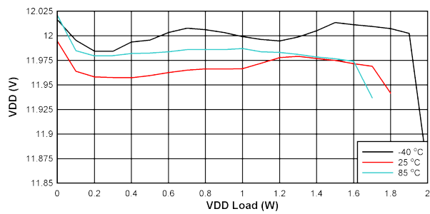
Figure 10-8. V_{DD-VEE} Load Regulation: V_{IN} = 12\text{ V} , V_{VDD-VEE} = 12\text{ V} , V_{COM-VEE} = 5\text{ V}
