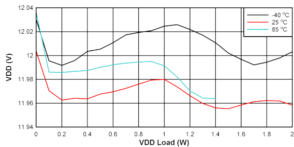
Figure 10-10. V_{DD-VEE} Load Regulation: V_{IN} = 18\text{ V} , V_{VDD-VEE} = 12\text{ V} , V_{COM-VEE} = 5\text{ V}
