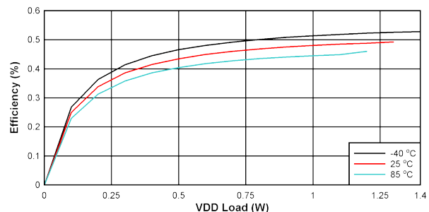
Figure 10-15. Efficiency vs Load on V_{DD-VEE} : V_{IN} = 10\text{ V} , V_{VDD-VEE} = 12\text{ V} , V_{COM-VEE} = 5\text{ V} , No Load on V_{COM-VEE}
