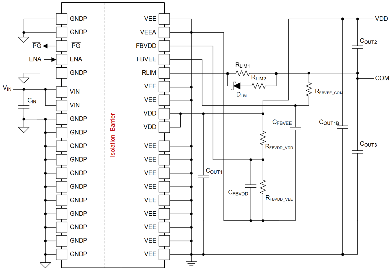
Figure 12-9. Dual output application schematic configured for V_{\text{COM\_VEE}} regulation = 2.5V
