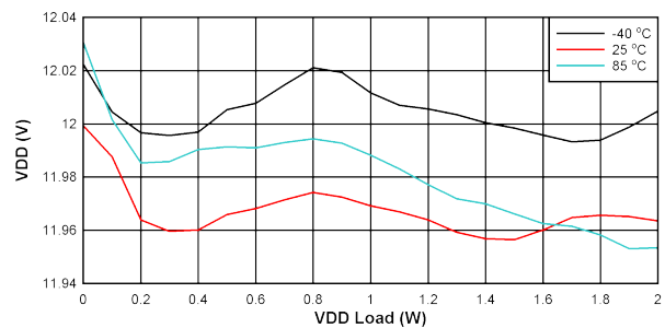
Figure 10-9. V_{DD-VEE} Load Regulation: V_{IN} = 15\text{ V} , V_{VDD-VEE} = 12\text{ V} , V_{COM-VEE} = 5\text{ V}
