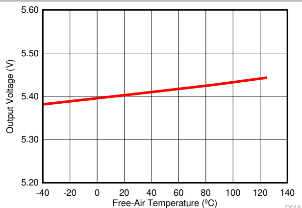
Figure 6-21. Isolated Supply Voltage ( V_{ISO} ) vs Free-Air Temperature
