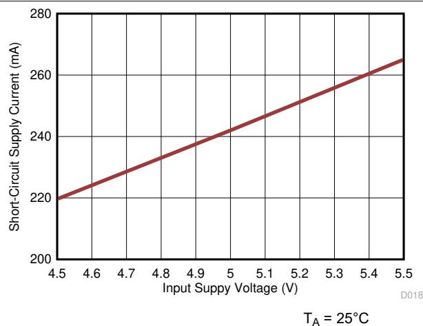
Figure 6-24. Short-Circuit Supply Current ( I_{INP\_SC} ) vs Supply Voltage ( V_{INP} )
