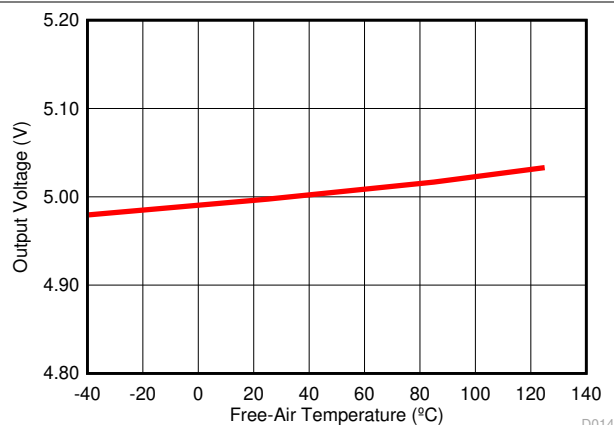
Figure 6-20. Isolated Supply Voltage ( V_{ISO} ) vs Free-Air Temperature
