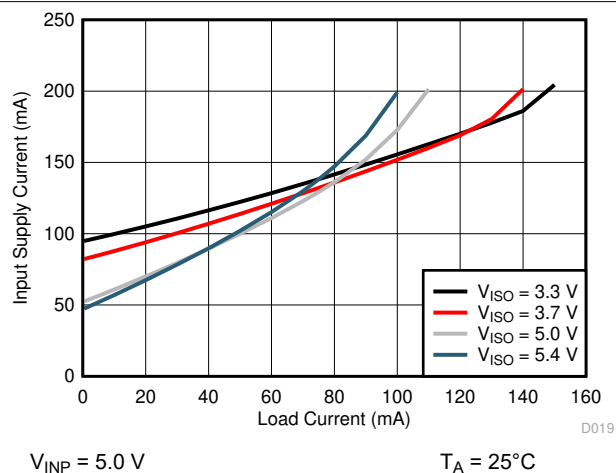
Figure 6-25. Input Supply Current ( I_{INP} ) vs Load Current ( I_{ISO} )
