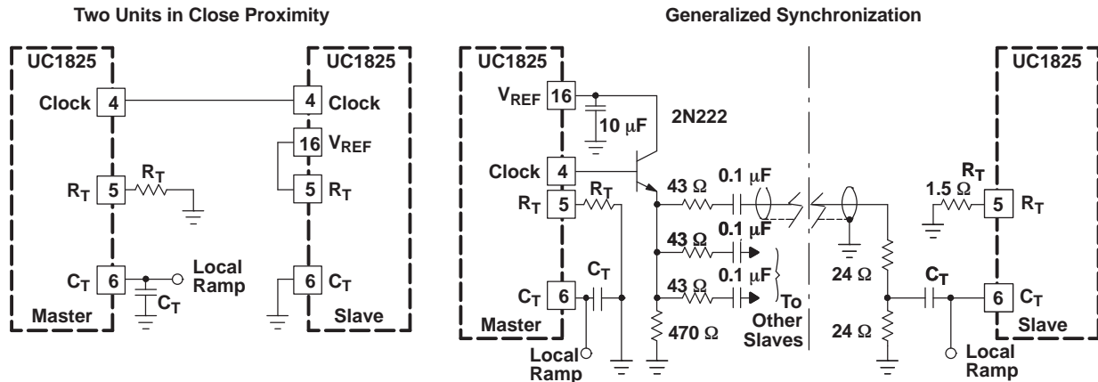
Figure 5. Synchronized Operation
