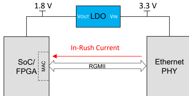
Figure 8-4. Residual Current Flowing Into MAC I/O Pins After PHY is Powered Up
