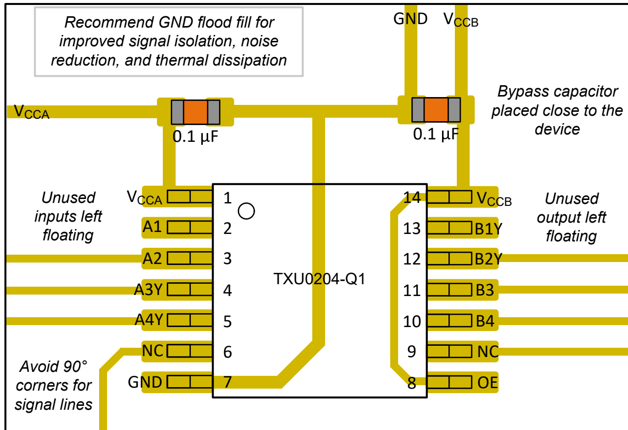
Figure 12-1. Layout Example – TXU0204-Q1
