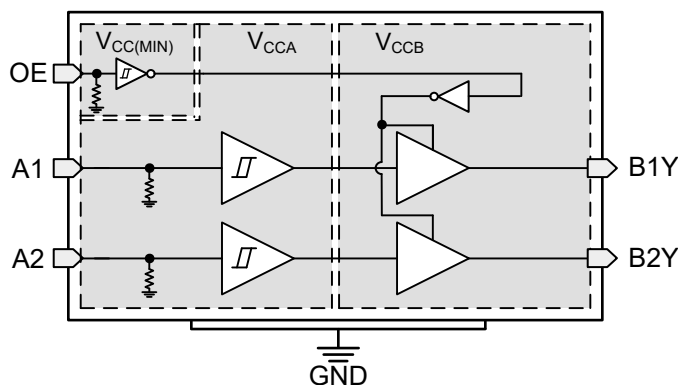
TXU0102 Functional Block Diagram
